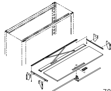
Portes escamotables
